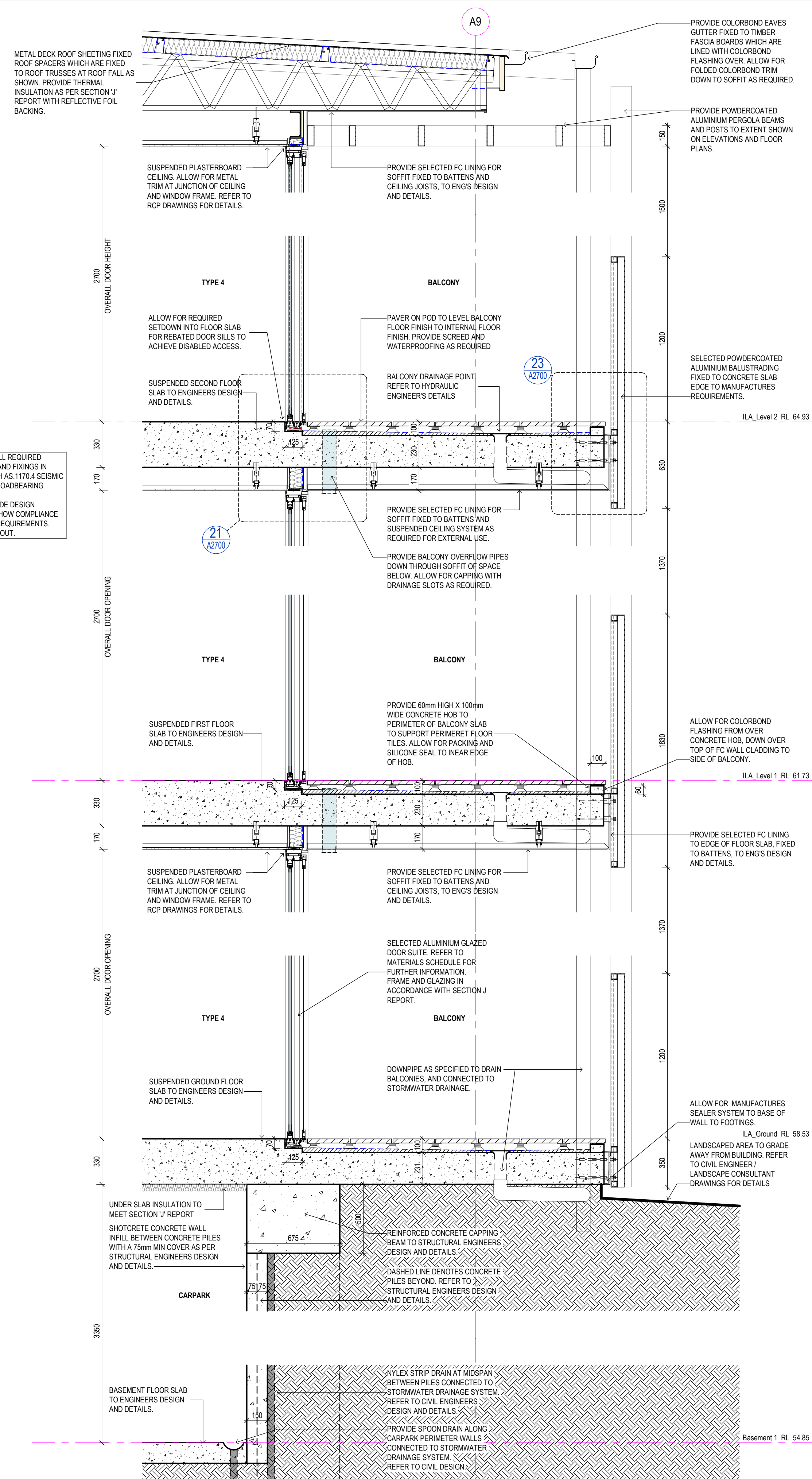
3 F ILA - WALL SECTION 03 Scale 1:20
